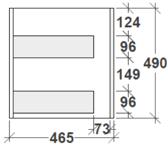
DOUBLE DRAWER SIDE VIEW
